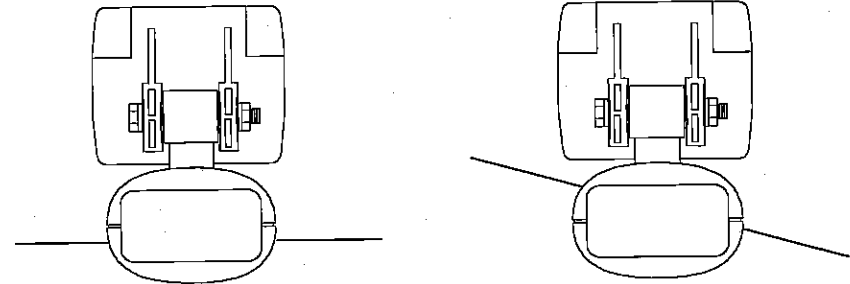
DEEP-VEE HULL
