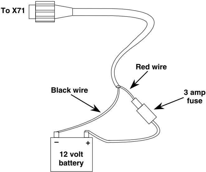
Power connections for the X71 sonar unit.
