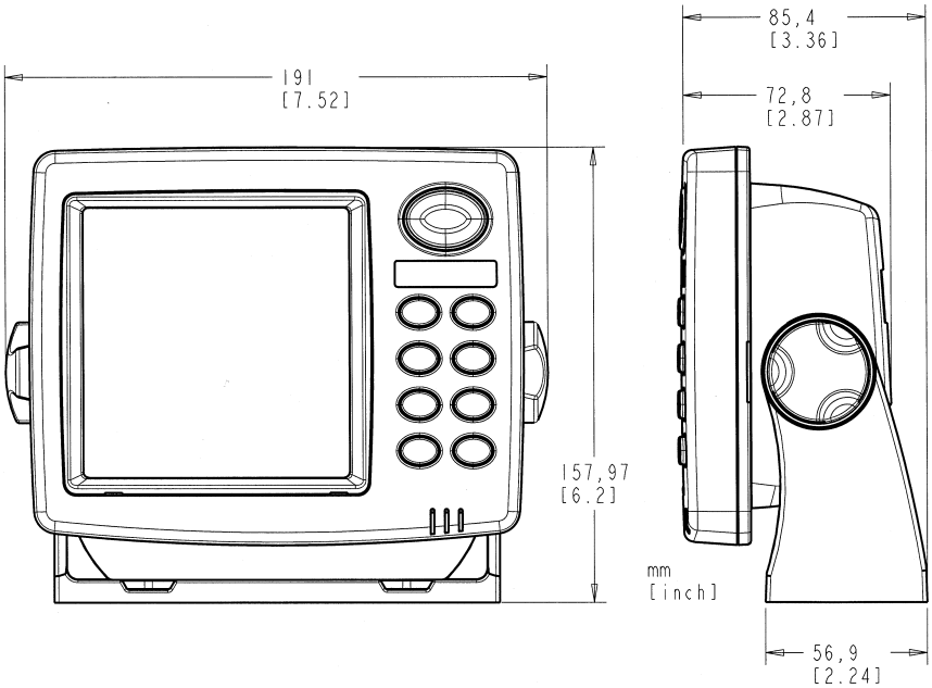
Front view (left) and side view (right) showing dimensions of X71 sonar unit when mounted on gimbal bracket.
