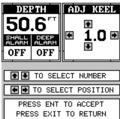
Keel Offset adjustment screen, set to one foot. Note how the digital depth display changed by one foot.
