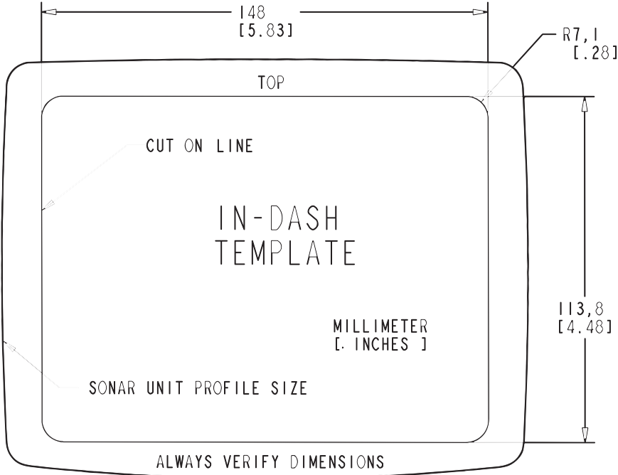
In-dash mounting template for X71 sonar unit, showing dimensions. NOTE: The figure above is not printed to scale. A scaled template is available for free download from our web site, www.lowrance.com .
